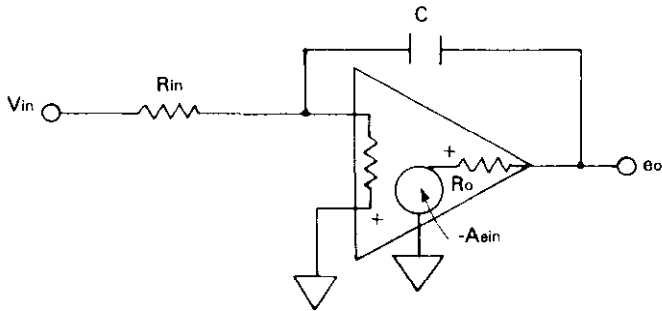
FIGURE 4-12. Integrator
